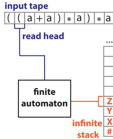
pushdown automaton
